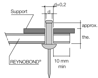
Riveting without expansion
