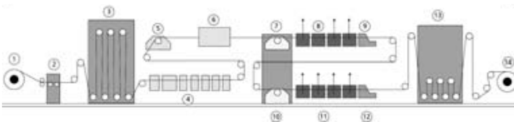
Diagram of the coil-coating line
