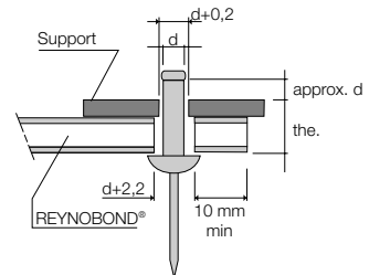
Riveting with expansion
